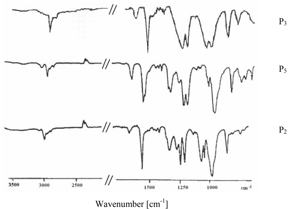
Figure 1. The IR spectra of the polyphosphates P 2 , P 3 and P 5
