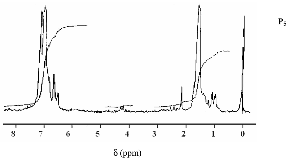
Figure 2. The ^1\text{H-NMR} -spectrum of polyphosphates \text{P}_1 and \text{P}_5
