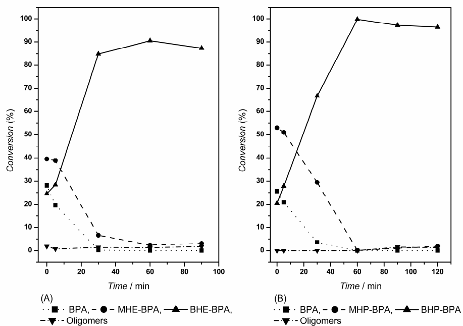
Fig. 1: Conversion of (A) BHE-BPA and (B) BHP-BPA
