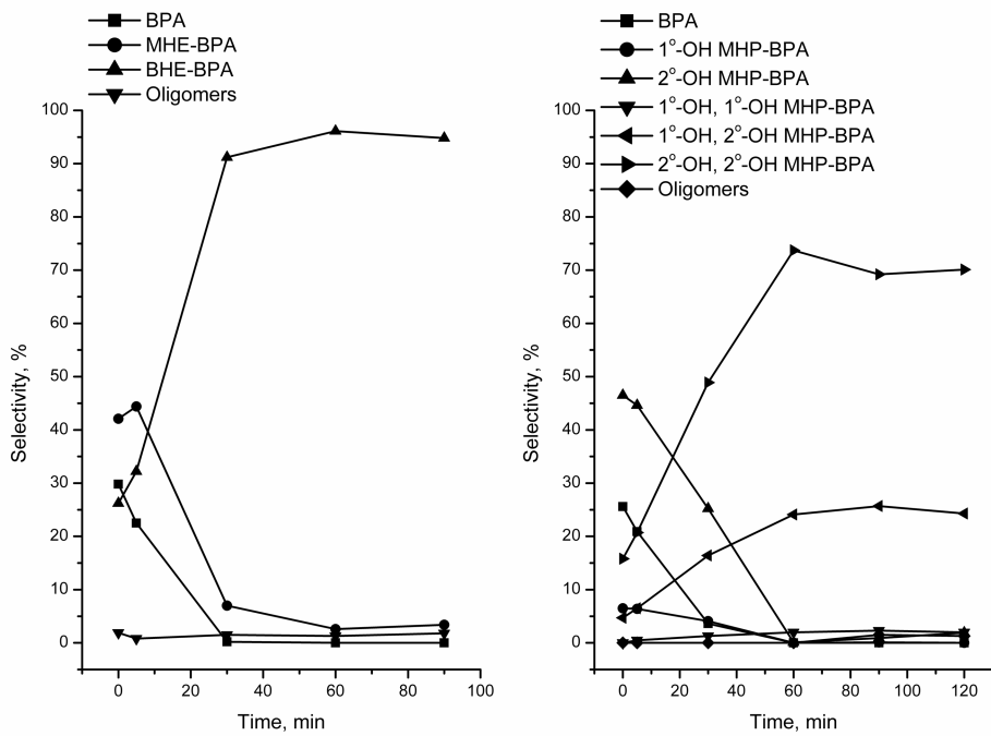
Fig. 2: Selectivity of (A) BHE-BPA and (B) BHP-BPA
