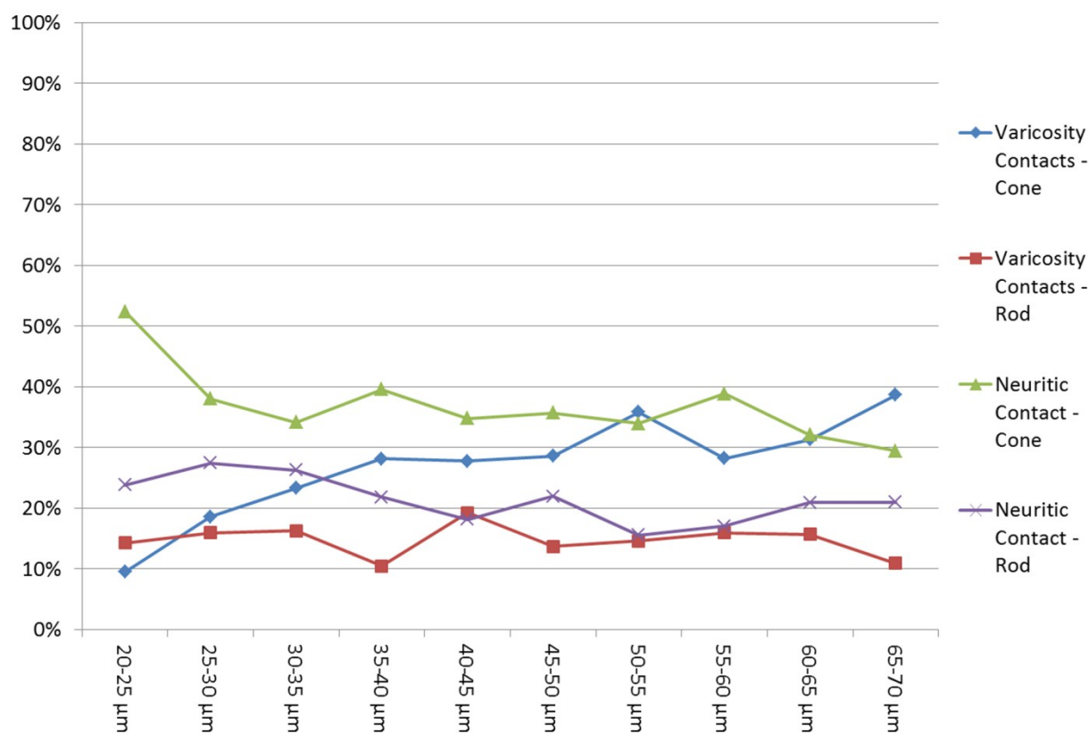
Supp. Fig. 1: Percentage of neuritic contacts (green and purple lines) and varicosity-containing neuritic contacts (blue and red lines) between rod or cone photoreceptor and target cell versus the distance between the photoreceptor and target cell.
