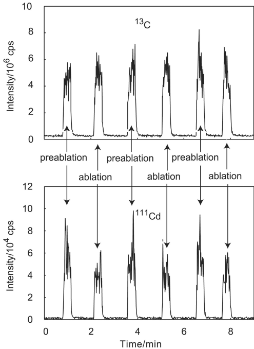
Fig A. Pre-ablation effect on ^{13}\text{C} and ^{111}\text{Cd} signal intensities in NIES 10b.
