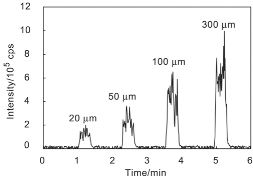
Fig B. Spot size effect on ^{111}\text{Cd} signal intensities in NIES 10b.
