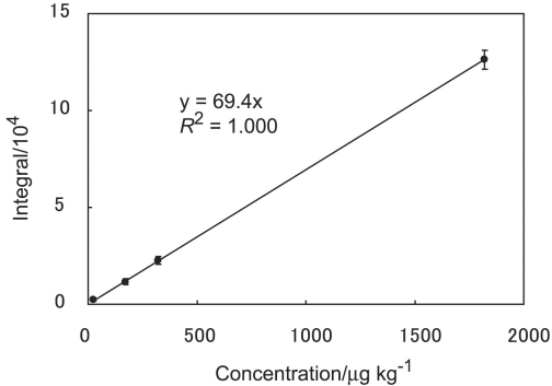
Fig. C Calibration line of integral intensity for ^{111}\text{Cd} using the selected reference materials. The error bars represent the standard deviation of 6 measurements.
