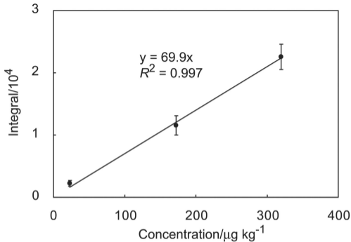
Fig. D Calibration line of integral intensity for ^{111}\text{Cd} using the selected reference materials in the sub \text{mg kg}^{-1} range. The error bars represent the standard deviation of 6 measurements.
