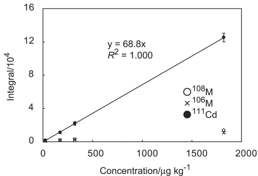
Fig. E Calibration line of integral intensity for 111 Cd after the correction of MoO interferences. The error bars represent the standard deviation of 6 measurements. 108 M and 106 M are integral intensities at m/z 108 and 106, respectively.
