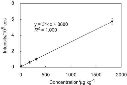
Fig. F Calibration line of signal intensity for ^{111}\text{Cd} after the correction of MoO interferences. The error bars represent the standard deviation of 6 measurements.
