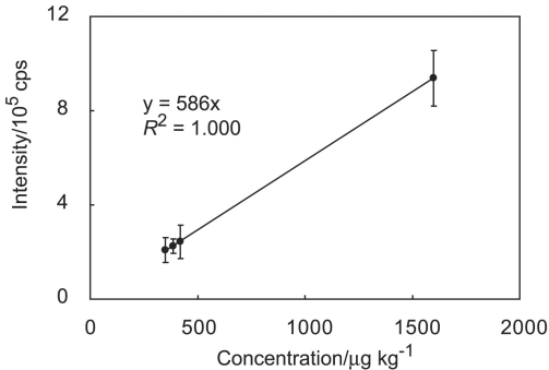
Fig. G Calibration line of signal intensity for 98 Mo using the selected reference materials. The error bars represent the standard deviation of 6 measurements. Using this calibration line, Mo in NIST 1568a was calculated to be 1.44 mg kg -1 , which was 99% of the certified value.
