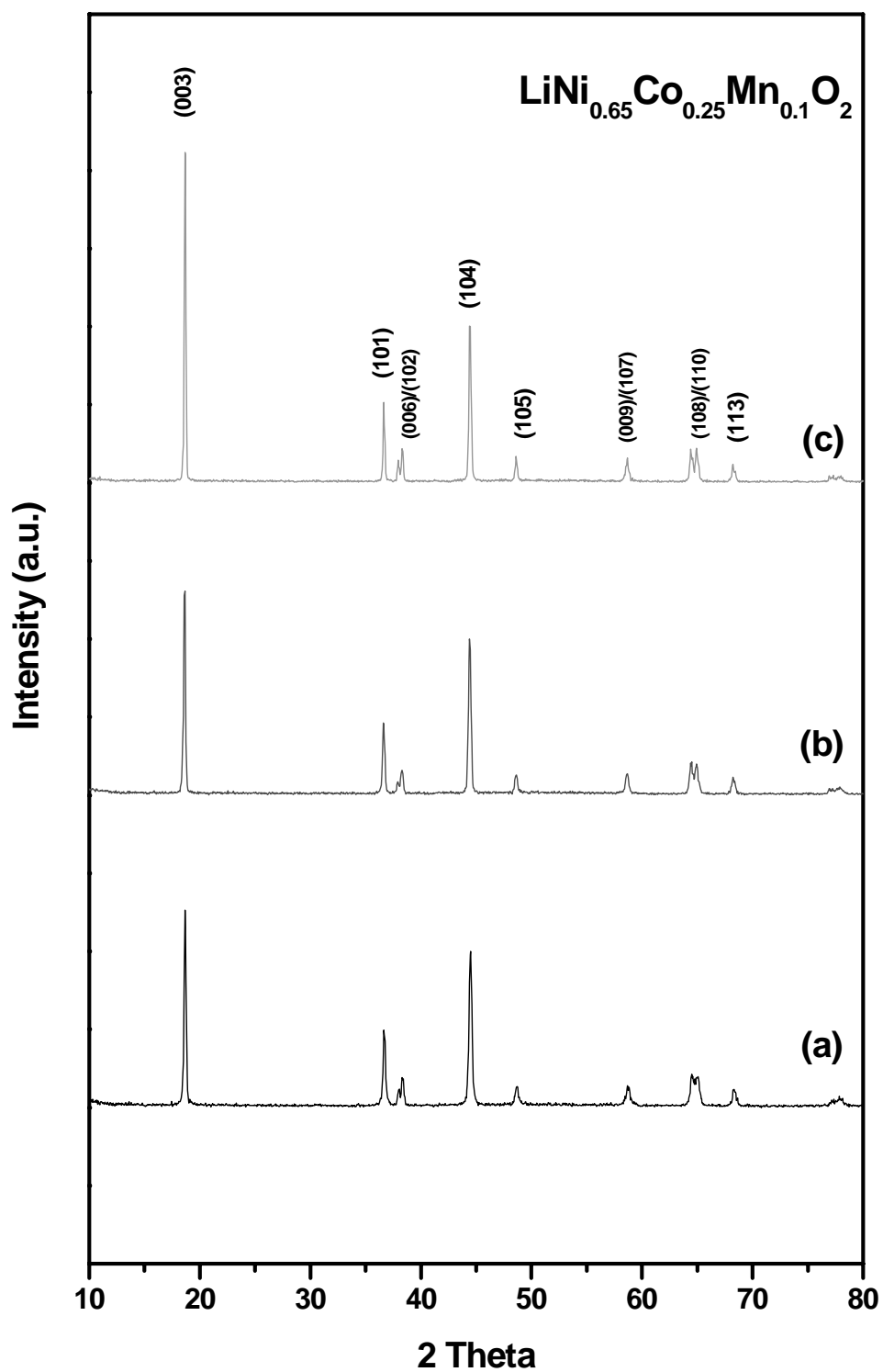
Powder XRD patterns of \text{LiNi}_{0.65}\text{Co}_{0.25}\text{Mn}_{0.1}\text{O}_2 sintered at (a) 800, (b) 850 and (c) 900°C for 12 h.
