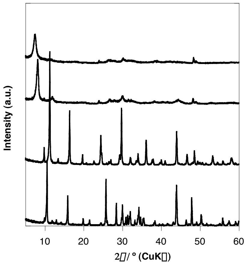
Figure S1. XRD patterns of (a) the starting material \text{Na}_2\text{Ti}_3\text{O}_7 , (b) \text{H}/\text{Ti}_3\text{O}_7 , (c) \text{MA}/\text{Ti}_3\text{O}_7 and (d) \text{PA}/\text{Ti}_3\text{O}_7 .
