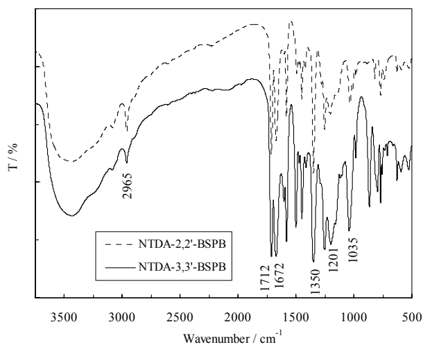
Fig. S2 IR spectra of NTDA-BSPB membranes.
