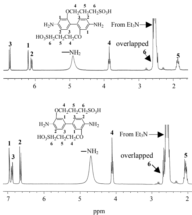
Fig. S1 1 HNMR spectra of BSPB diamine monomers.
