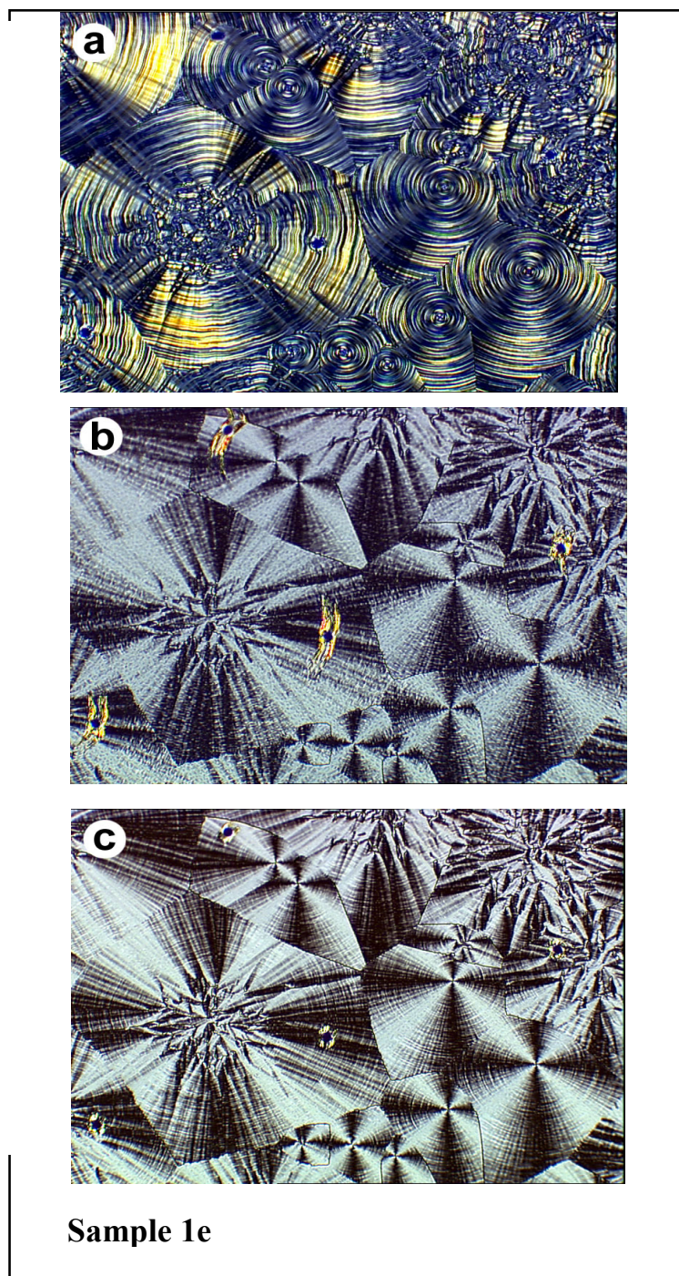
Figure 7: Optical texture of Sample 1e (a) with +20\text{V}/\mu\text{m} , (b) no field, and (c) with -20\text{ V}/\mu\text{m} .
