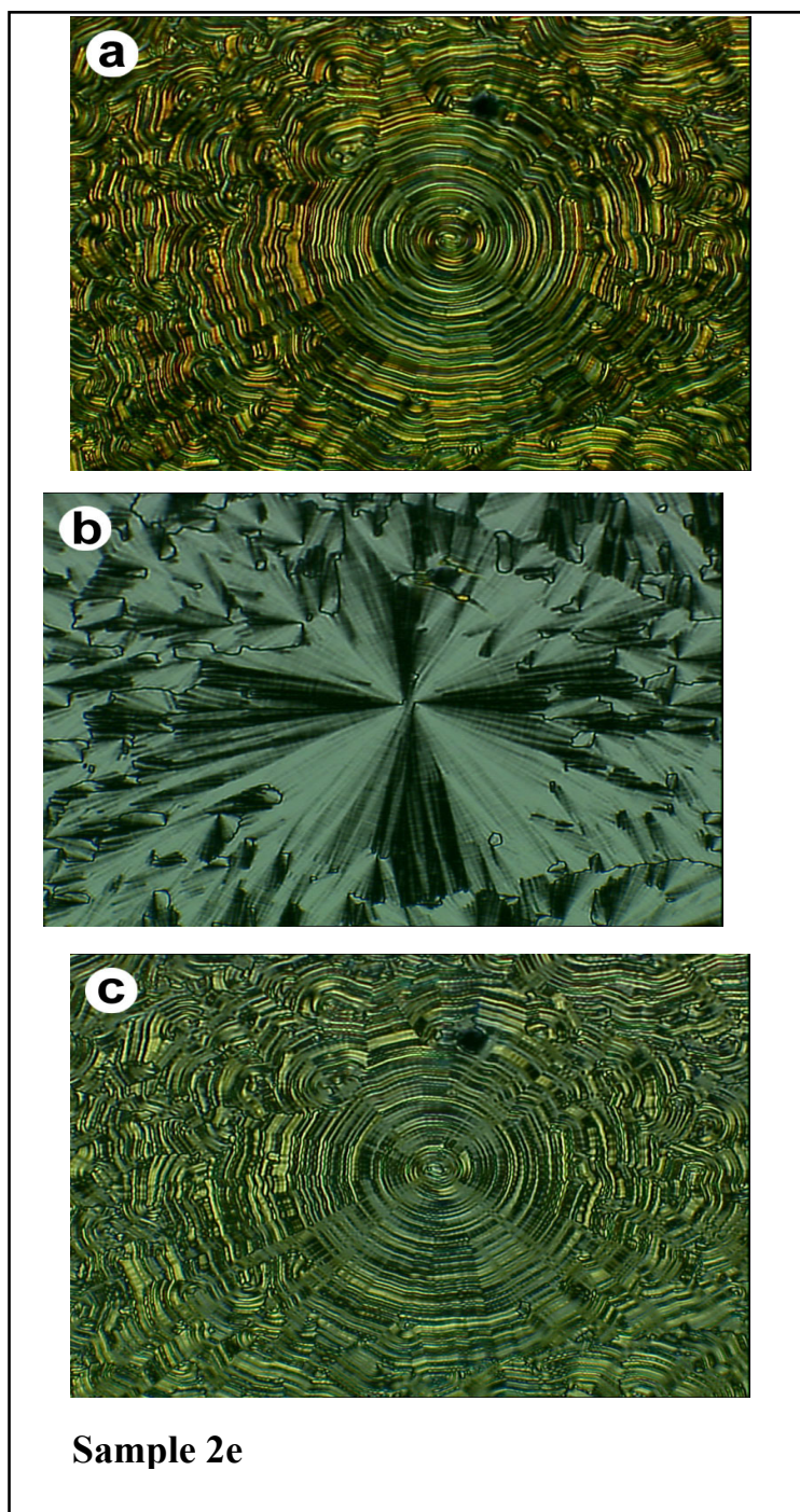
Fig. 8: Optical texture of Sample 2e (a) with an applied field of +20\text{V}/\mu\text{m} , (b) without field (c) with -20\text{V}/\mu\text{m} . Polarizer/analyzer is parallel/perpendicular to the image frame.
