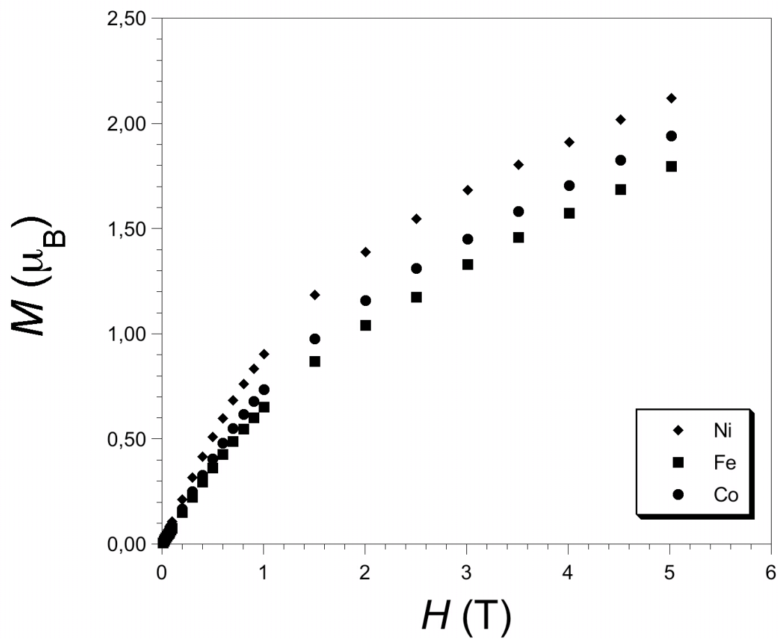
Fig. S3 Field dependence of the magnetization for compounds 3-5 .
