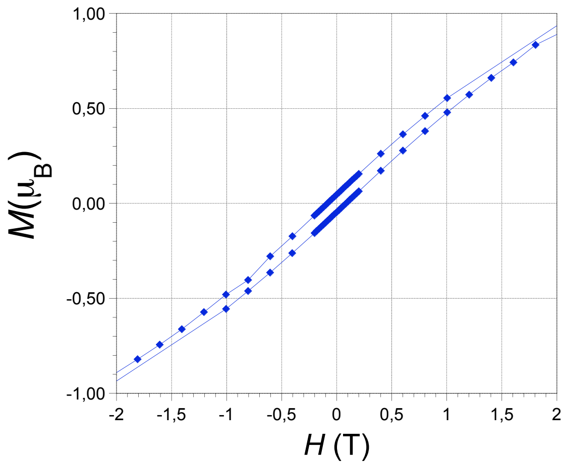
Fig. S4. Magnetic hysteresis at 2 K for compound 5.
