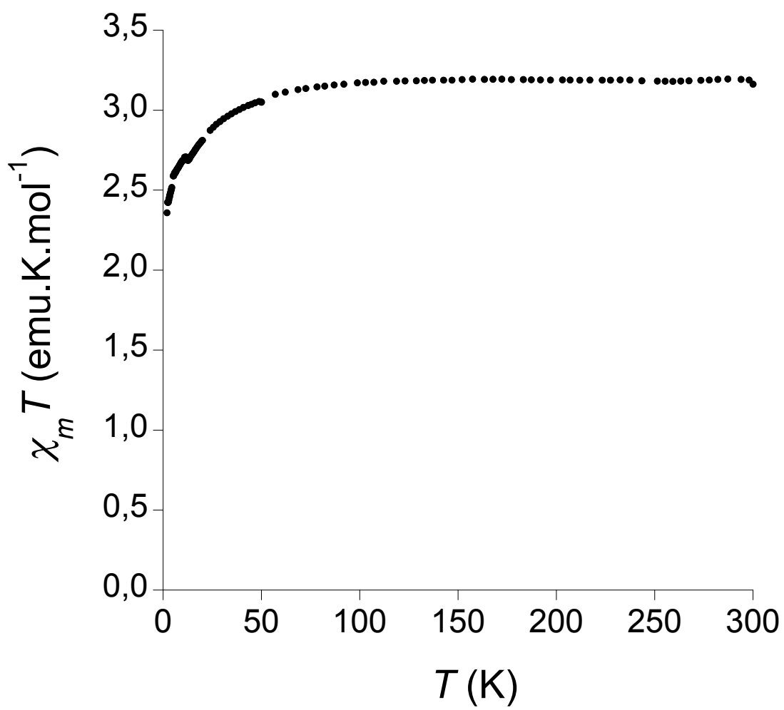
Fig. S2 Thermal dependence of the \chi_m T product for compound 2 .
