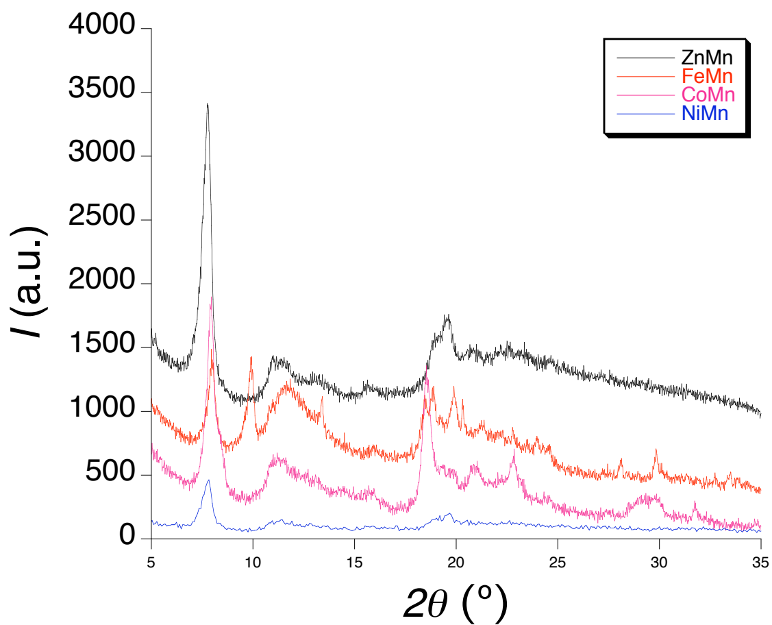
Fig. S1. X-ray powder patterns for compounds 2-5.
