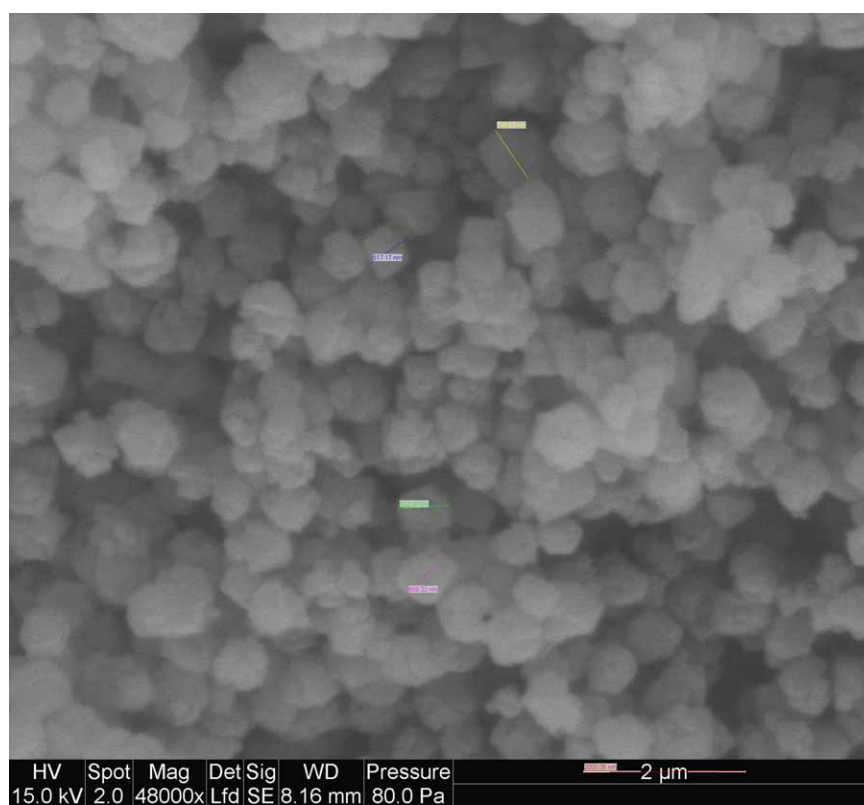
SEM Image of Zeolite Y powder used for comparison.
