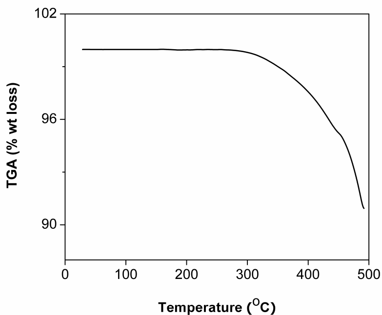
Figure 1. TGA curve of the BPTBTD powder.
