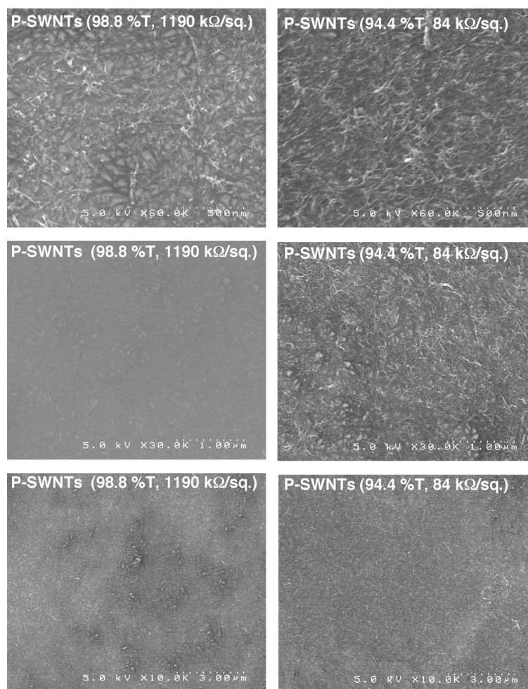
Figure S2. SEM images of P-SWNTs on a PET film.
