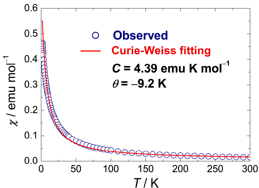
Figure S1. Temperature-dependent magnetic susceptibility ( \chi ) of 2_2\text{FeCl}_4(\text{DCE}) .
