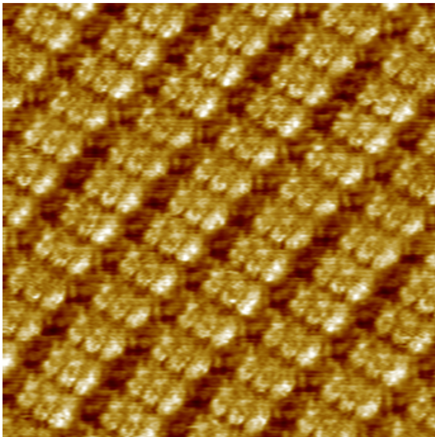
STM image of O3A at the n-tetradecane/HOPG interface ( 15 \times 15 \text{ nm}^2 ; I_t=86 \text{ pA} ; V_t=400 \text{ mV} ).
