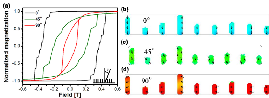
Figure A: Micromagnetic simulations of an array of aligned Fe nanowires with several heights. (a) Hysteresis curves of the external magnetic field applied at 0°, 45° and 90° with respect to the nanowire axis. Vector field of the magnetization in the Fe particle array with the external magnetic field applied at (b) 0°, (c) 45° and (d) 90° with respect to the particle axis.
