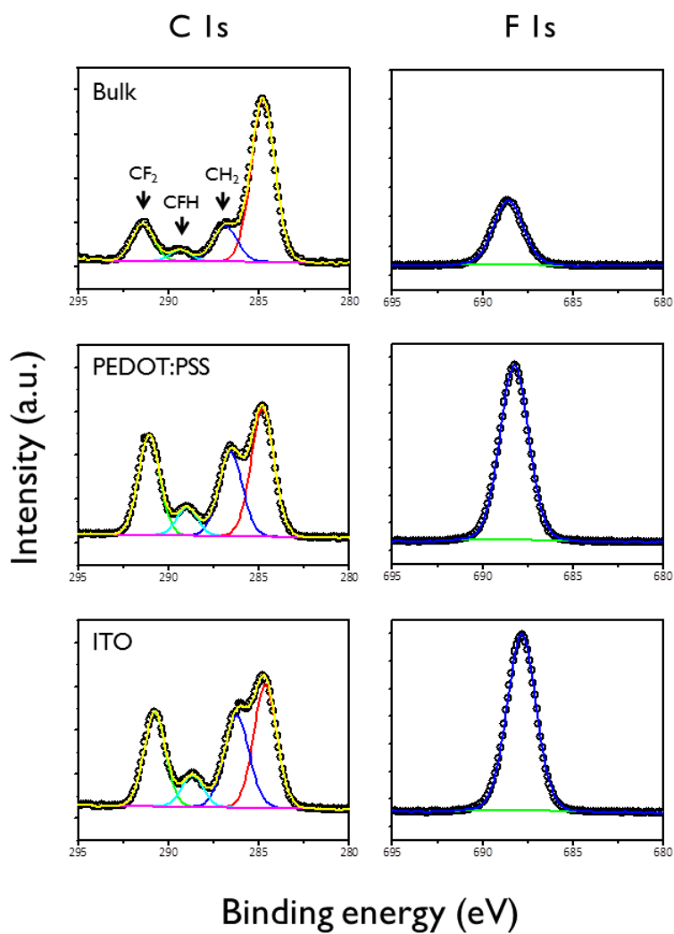
Figure S3. Fitting results of XPS spectra of all samples: (left) C 1s and (right) F 1s.
