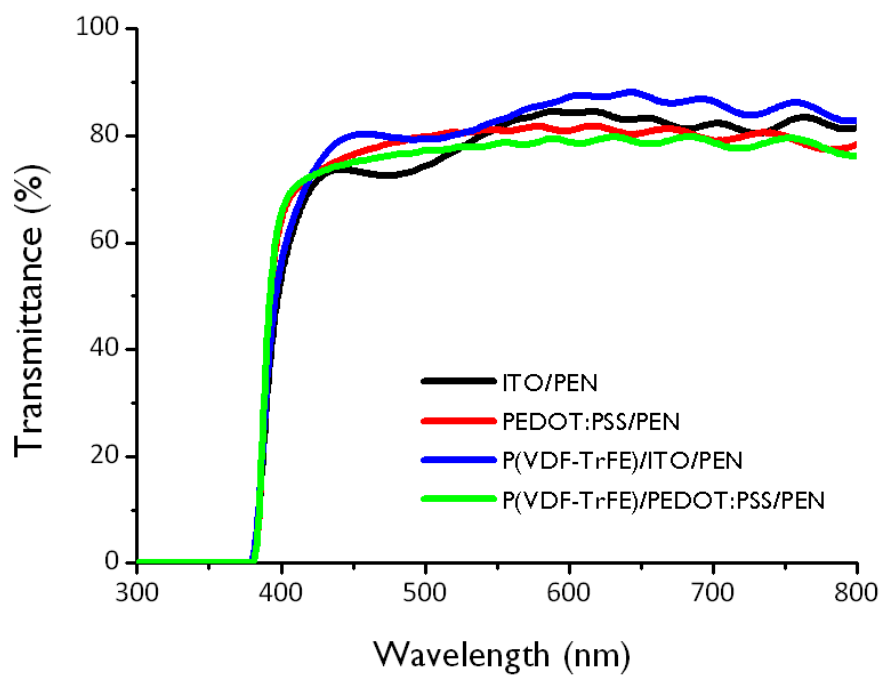
Figure S2. Transmittance of all flexible samples used in this study.
