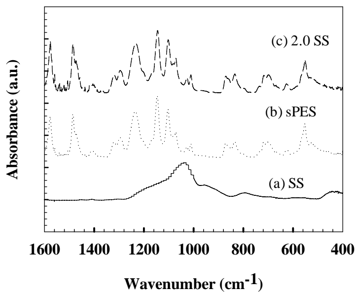
Fig.S1 Representative IR spectra of (a) inorganic filler, SS, (b) pristine membrane, sPES, and (c) composite membrane with 2 wt% SS.
