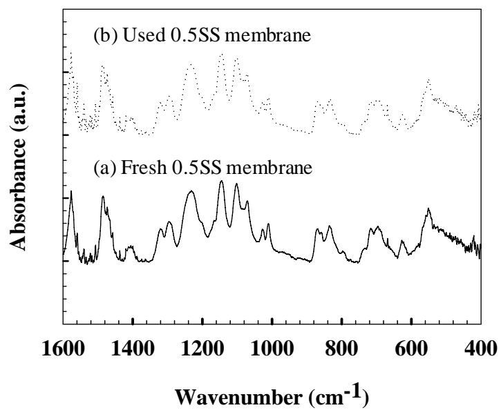
Fig.S2 IR spectra of (a) fresh and (b) used composite membrane with 0.5 wt% SS.
