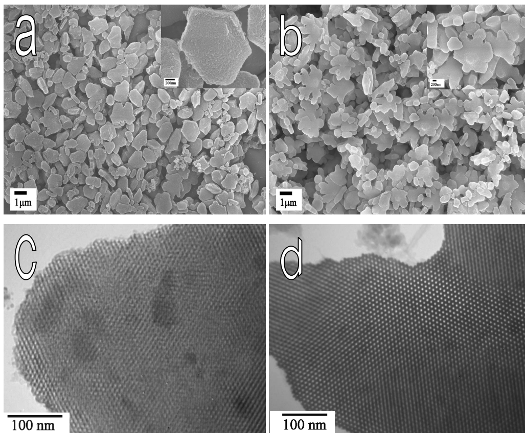
Fig. S1 (a) SEM image of S3; (b) SEM image of S4; (c) TEM image of S3; (d) TEM image of S4.
