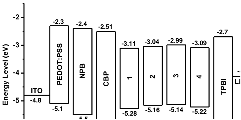
Fig S2. Energy level diagram of the materials used in the devices.
