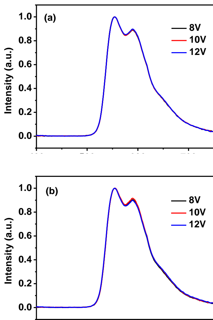
Fig. S1 Normalized EL spectra of complex 4 in device I (a) and II (b) at different voltages.
