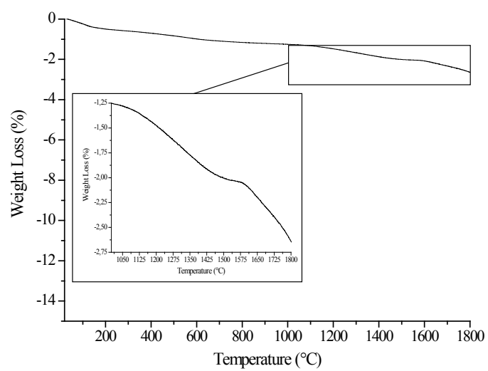
Figure 1SI. TGA curve recorded during annealing of sample 1 in nitrogen environment from RT to 1800 °C.
