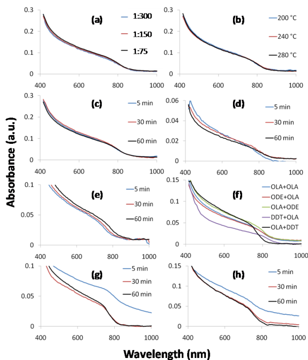
Fig. S1. UV-Vis spectra of (a) different precursors to OLA ratios (CIS1, CIS2 & CIS3), (b) different growth temperature (CIS2, CIS4 & CIS5), (c-e) CIS2, CIS1 & CIS4 analysed during the reaction at different time intervals to monitor the progress of reaction (f) different capping agents (CIS2, CIS6, CIS7, CIS8 and CIS9), (g & h) CIS9, CIS8 samples analysed at different time intervals during reaction.
