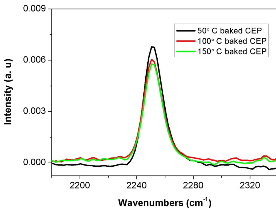
Electronic supplementary information B. FT-IR of CEP films baked at different temperatures.
