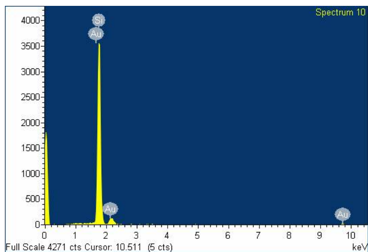
Figure S1. EDX spectrum of linear arrays with nanoparticle size of 5 nm indicates the existence of Au and Si elements.
