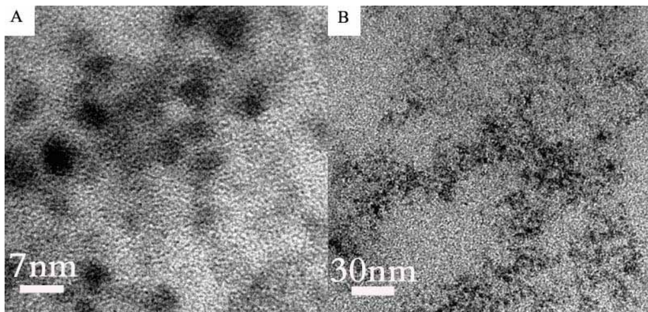
Figure S1. TEM images of Fe 3 O 4 -CdSe/CdS nanocomposites placed for 16 weeks.
