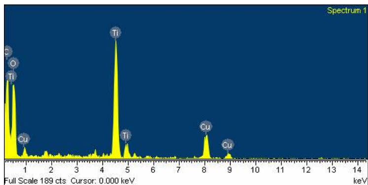
Fig. S1 Energy dispersive X-ray spectroscopy (EDS) of NS-Ti 4 O 7
