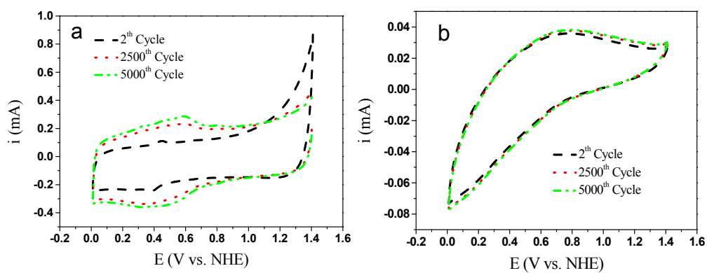
Fig.S2 CV plots of XC-72 (a) and Ti 4 O 7 (b) during electrochemical ADT tests
