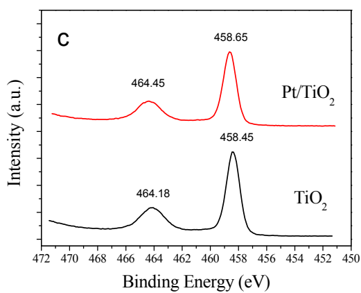
Fig. S4 XPS survey scans of TiO 2 (a) and Pt/TiO 2 (b) and XPS spectra of Ti 2p for TiO 2 and Pt/TiO 2 (c)
