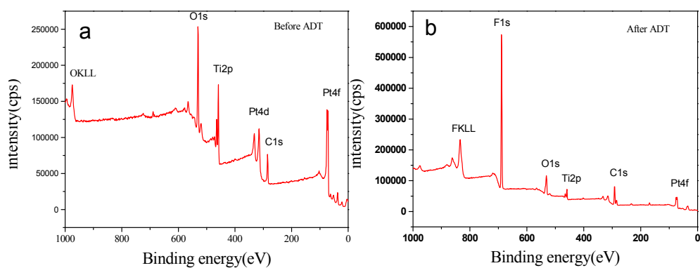
Fig. S3 XPS survey scans of Pt/NS-Ti 4 O 7 before(a) and after(b) ADT
