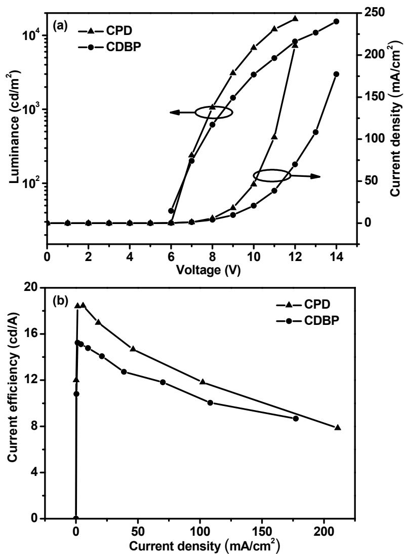
Figure S1. The current density-voltage-luminance ( J-V-L ) curves for the CPD and CDBP devices. The device structures are ITO/PEDOT:PSS (40 nm)/NPB (20 nm)/host:FIrpic (10wt%, 30 nm)/TPBI (40 nm)/LiF (1 nm)/Al (150 nm), in which host = CPD or CDBP.
