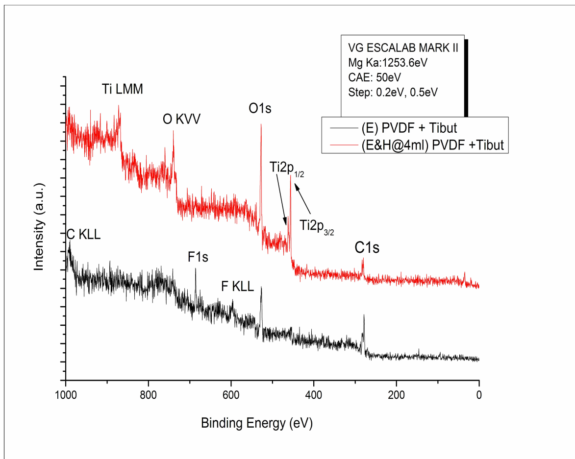
Figure: XPS spectra of (a) amorphous Ti at the electrospun PVDF nanowires core (black), crystallized TiO 2 on PVDF nanofibers after hydrothermally treated with 4ml (red)
