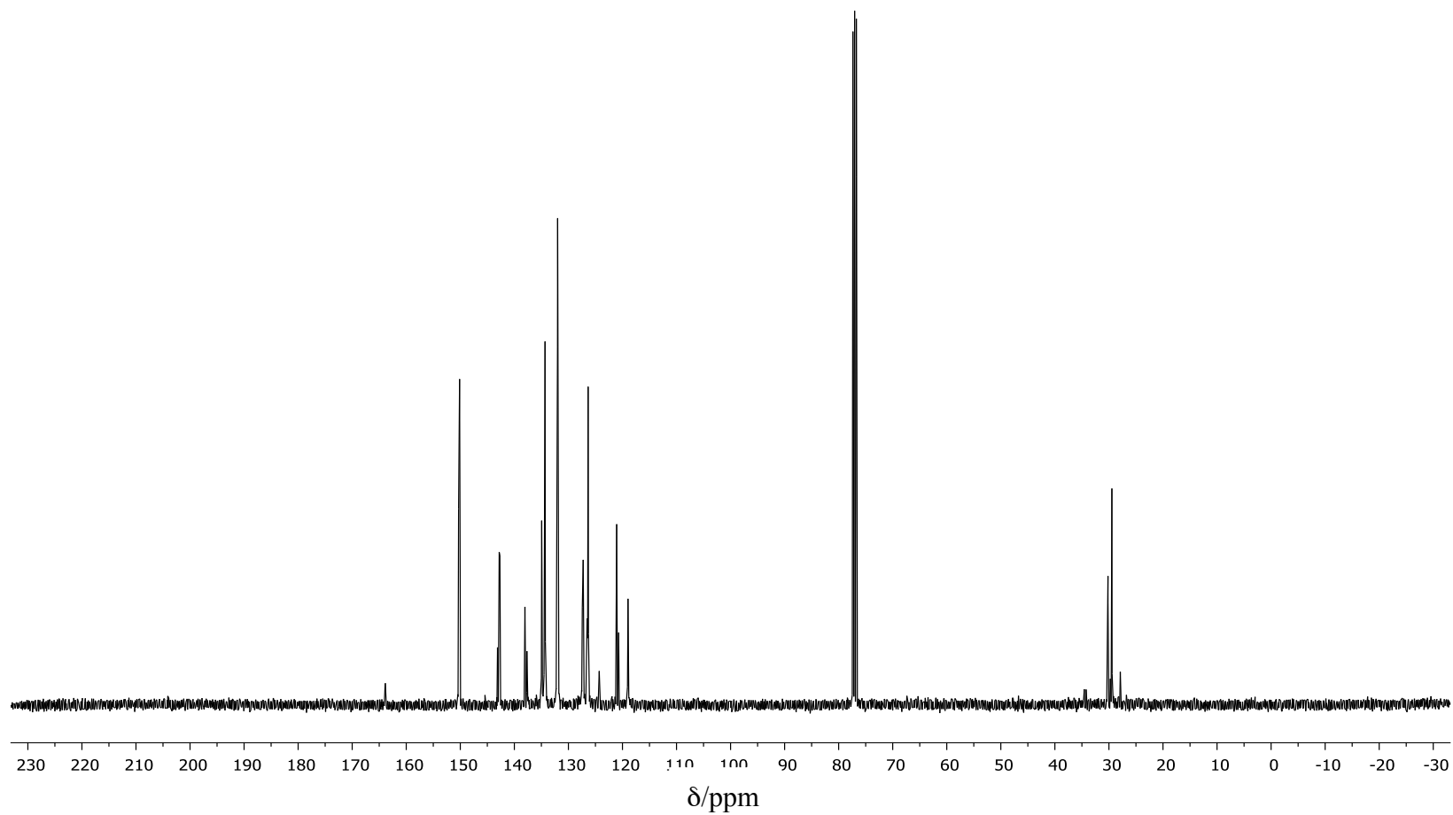
^{13}\text{C} -NMR spectrum of Zn-2 in \text{CDCl}_3 .
