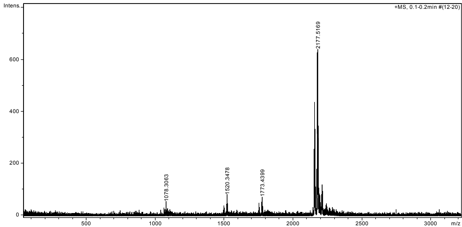
ESI-HRMS spectrum of Zn-1
