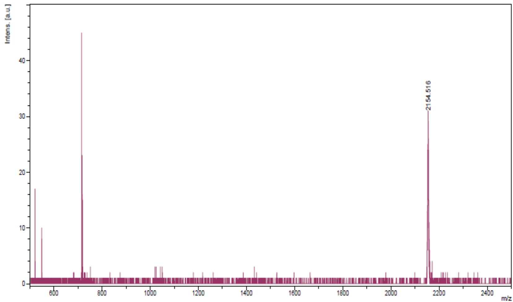
MALDI-TOF mass spectrum of Zn-2 .
