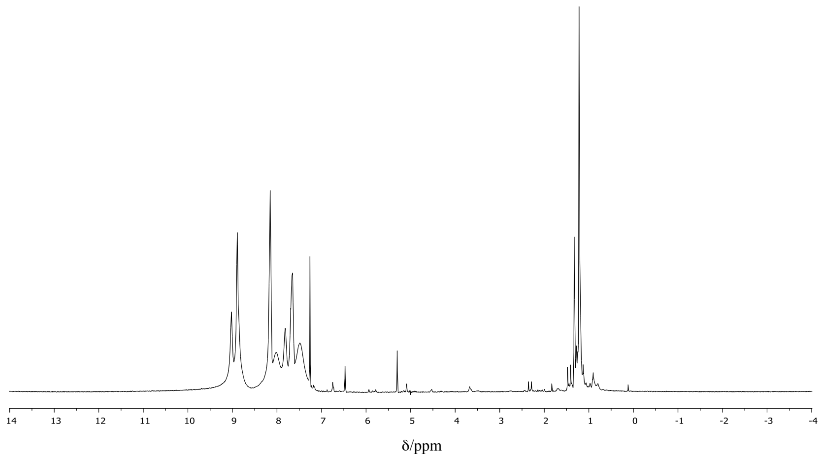
^1\text{H-NMR} spectrum of Zn-2 in \text{CDCl}_3
