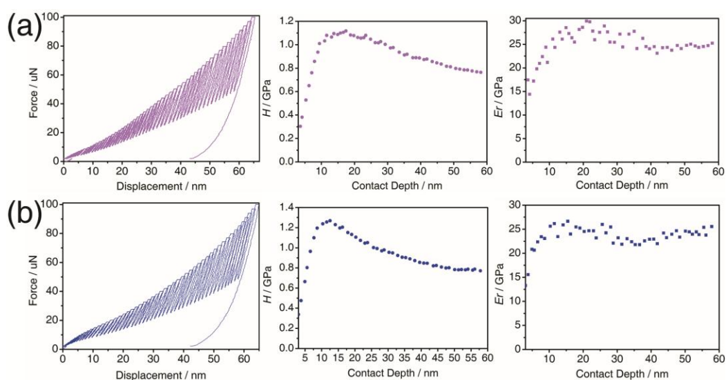
Fig. S1 (a, b) Two of the partial unloading nanoindentation results.
