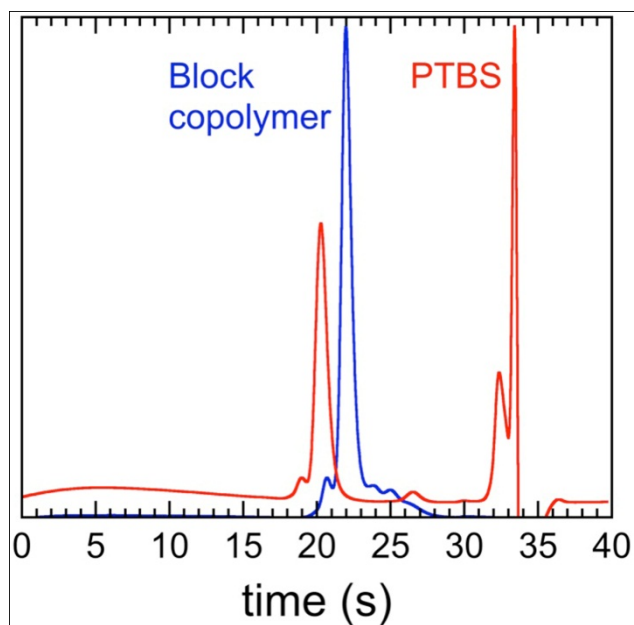
Figure S1. Refractive index (arbitrary units) elution results acquired from the block copolymer and PTBS homopolymer described in the text.
