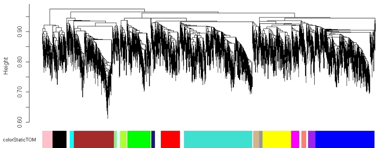
TCG Cluster Dendrogram
