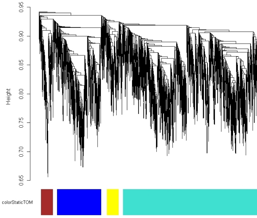
TCB Cluster Dendrogram
