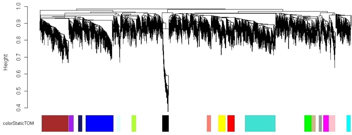
HCB Cluster Dendrogram
