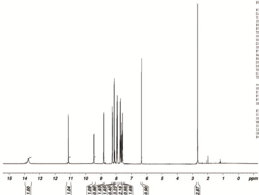
1 H NMR Spectrum of compound 6
