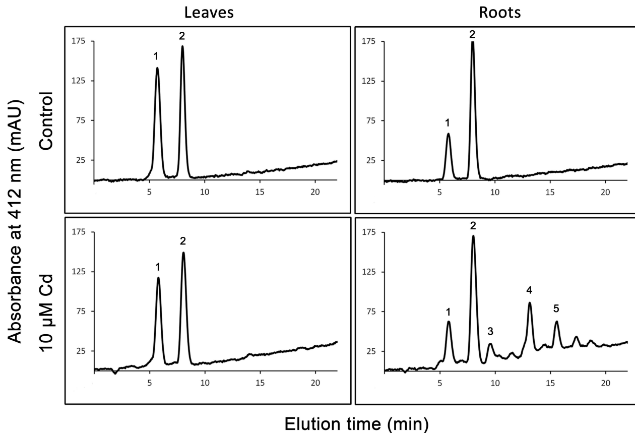
Figure S1. Biothiol profile of peanut plants treated with Cd 0 and 10 \mu M. Peaks were identified by the elution of commercially available standards. Concentration was calculated by the integration of the internal standard N-acetyl-cysteine (Peak 2): GSH (1), PC2 (3). PC3 (4)
