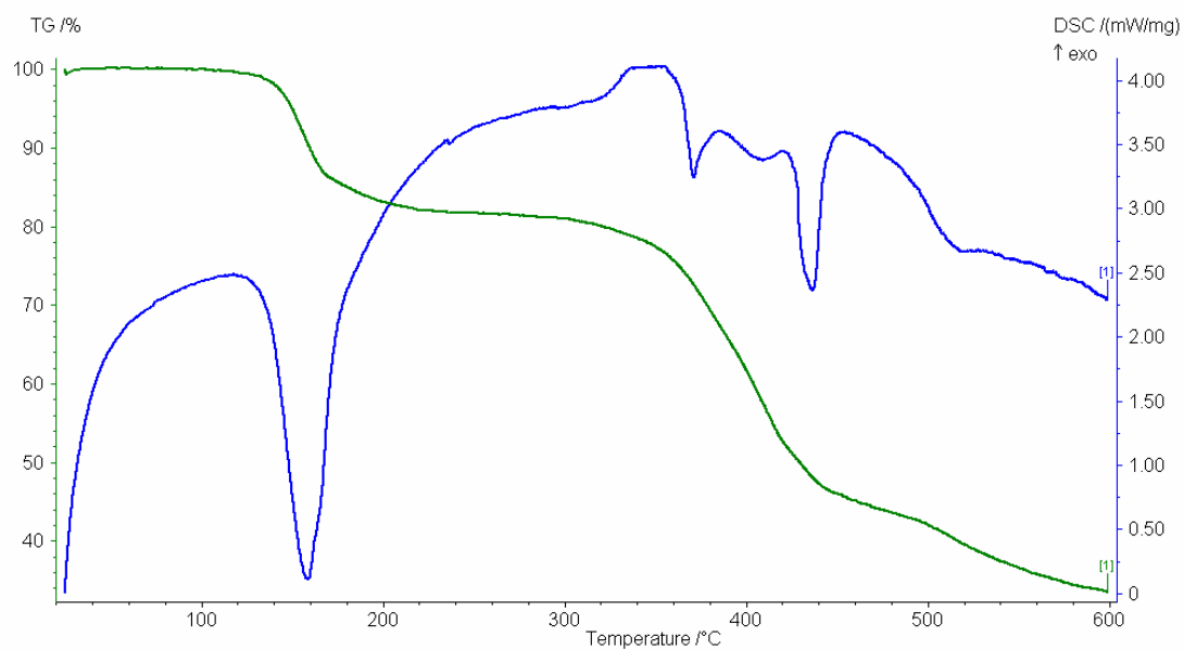
Fig. 2 TGA/DSC of complex 2
