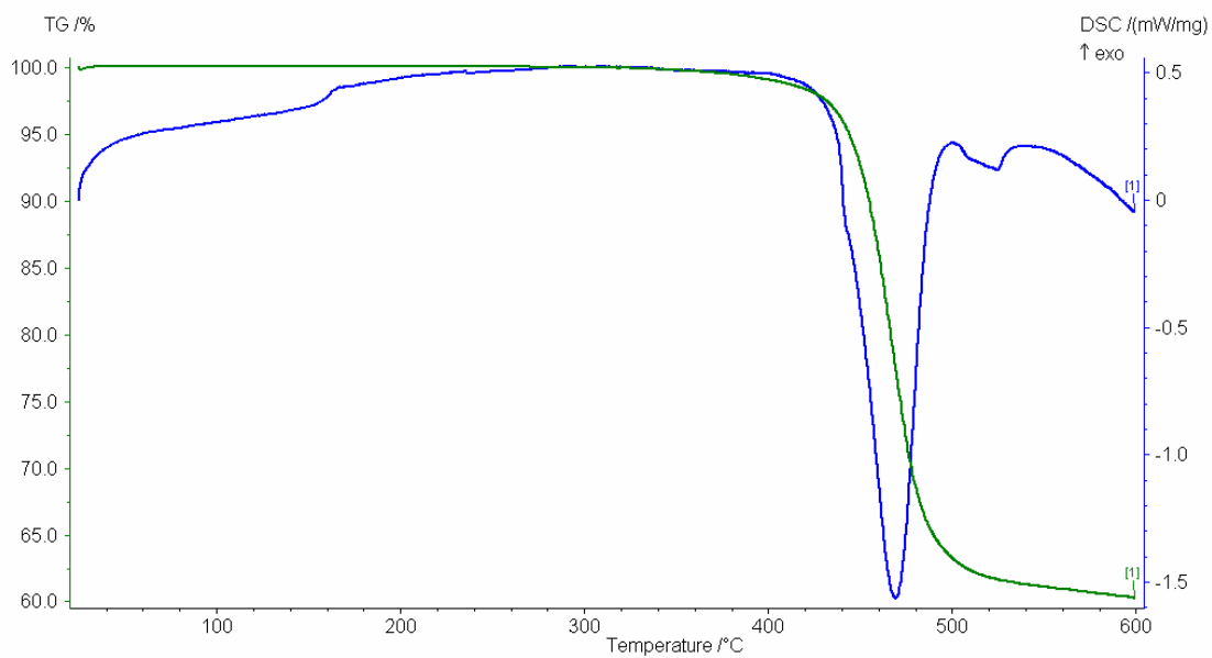
Fig. 1 TGA/DSC of complex 1
