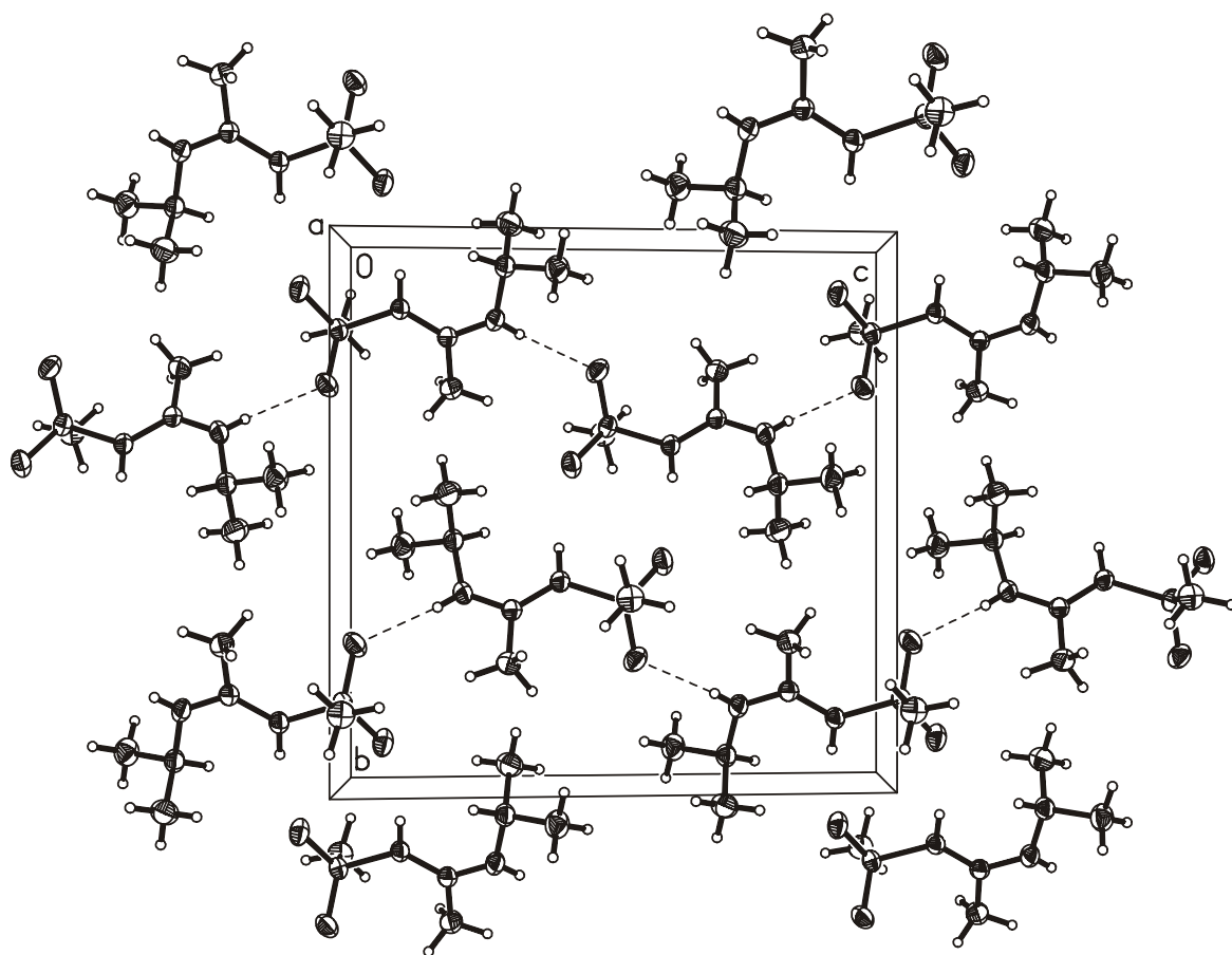
Fig. S1. The view of a crystal packing of 8 shown along the a-axis. Molecules form infinite hydrogen-bonded chains along the c-axis. The chains are interlinked with weak C(2)-H(2)⋯O(1) hydrogen bonds passing in perpendicular direction (not shown in the drawing).
