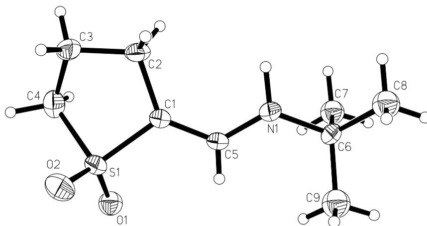
Fig S2. X-ray derived geometry of the sulphone 15
