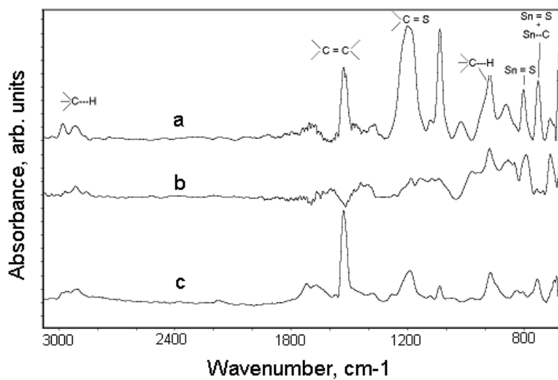
FTIR spectra of the deposits (a-c) obtained at respective conditions A, B and C (Table 1).
