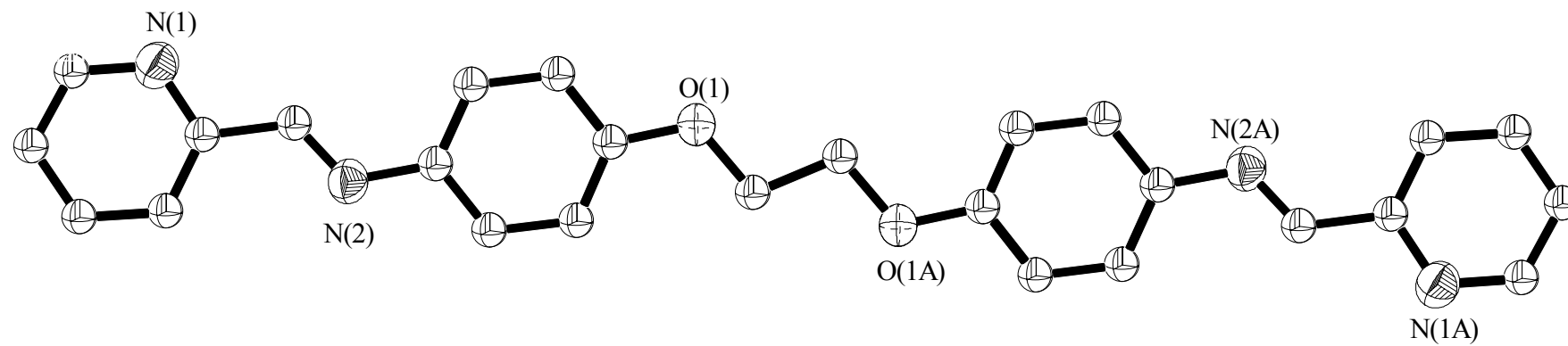
ORTEP plot of the ligand BL 6 . The hydrogen atoms and solvent molecule are omitted for clarity.
