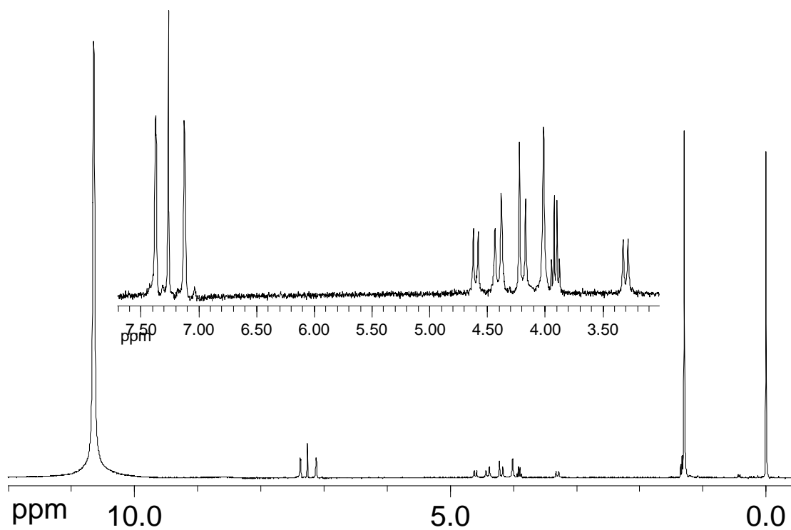
1 H NMR of compound 3 in pure CDCl 3 plus minor CF 3 COOH (produced by MestRec 4.27)
