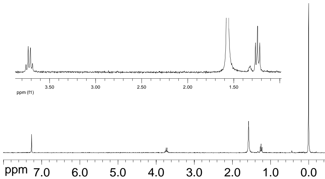
1 H NMR of compound 3 in pure CDCl 3 (produced by MestRec 4.27)
