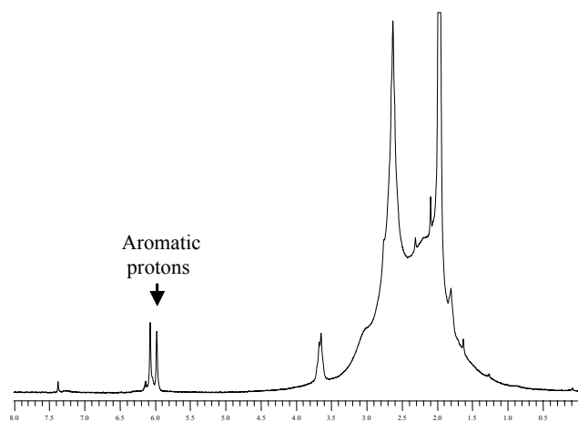
Fig 1S. 1 H NMR spectrum of CrPAN prepared from bis(benzene)chromium (CD 3 CN solution)
