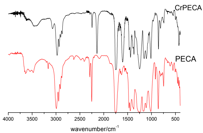
Fig. 2S. The IR spectra of CrPECA and PECA
