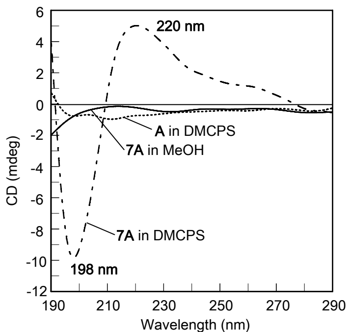
Figure 1S. CD spectra of 7+A in DMCPs gel (dotted) and MeOH solution (bold). [7+A] = 10 mg/mL.
