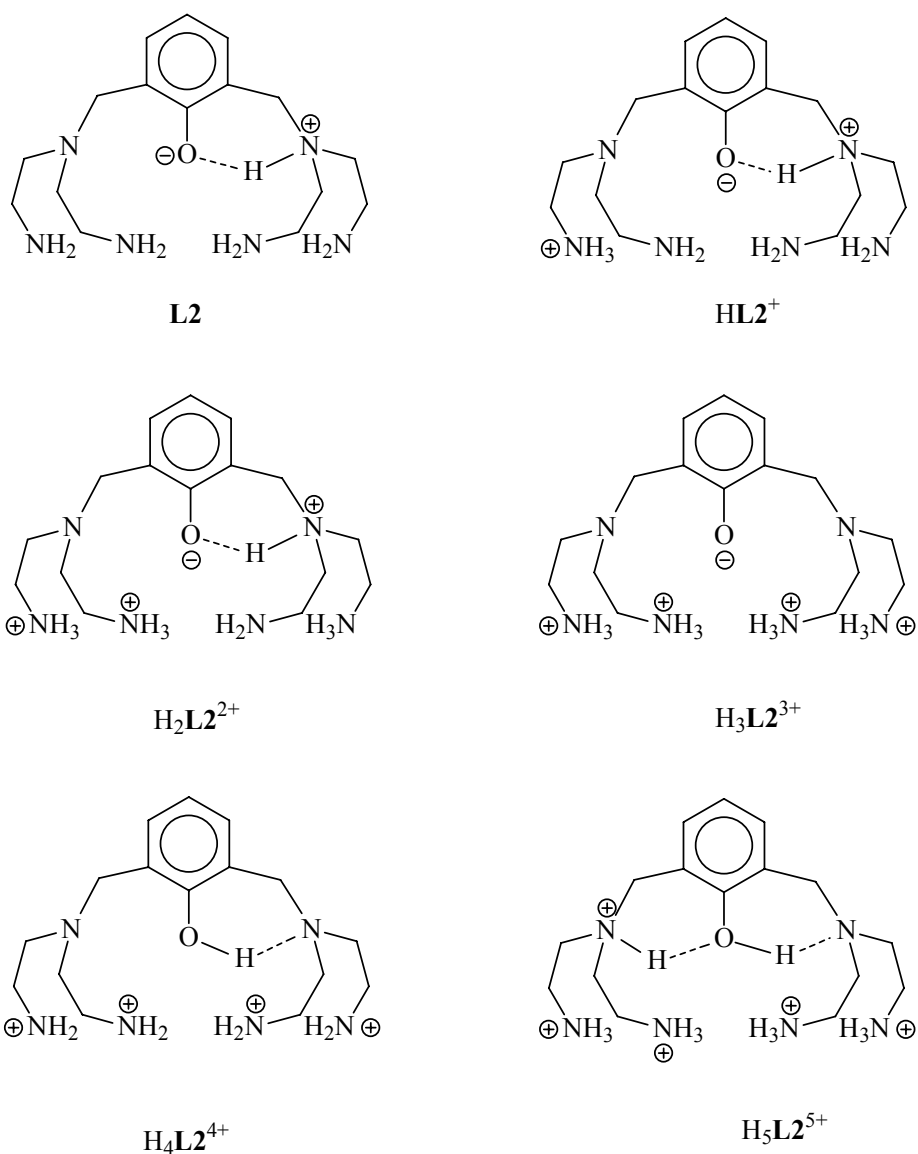
Figure S1 Location of acidic hydrogen atoms in the protonated species of L2
