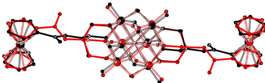
Figure S2. Superposition of the two crystallographically independent anion moieties in the structure of 2a (molecule 2 in red, molecule 1 in black).
