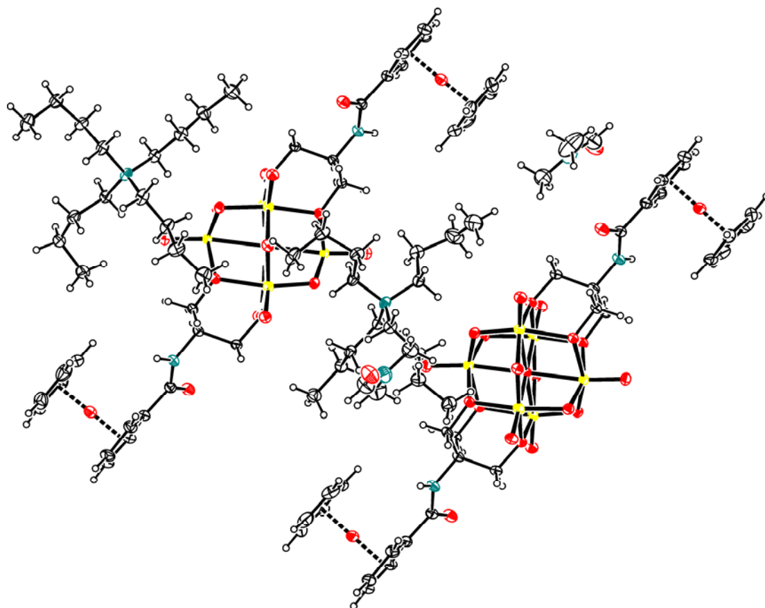
Figure S1. 'Full' PLATON plot of the structure of 2a .
