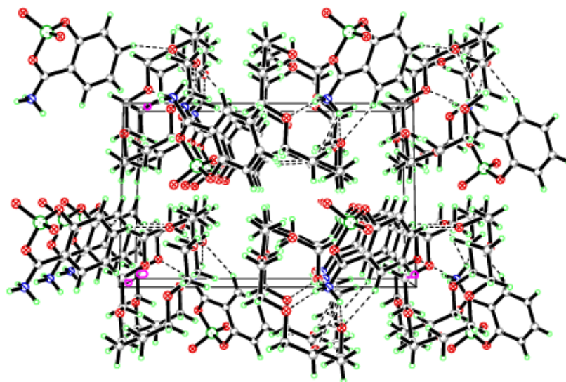
Fig. S4 3-D stacking motif of complexes 5
