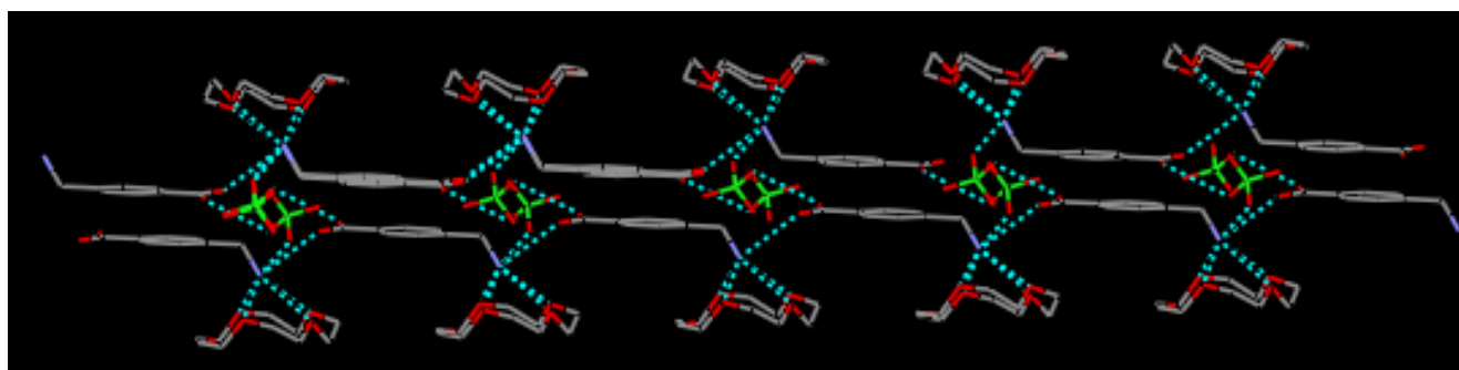
Fig.S1 1D connecting motif of complexes 2
