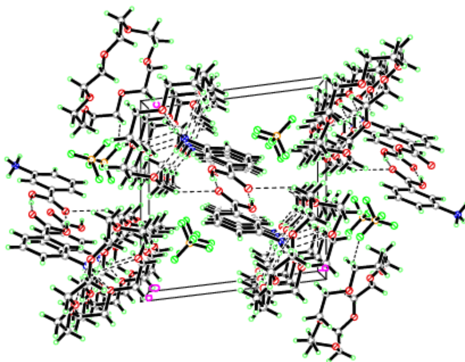
Fig. S3 3-D stacking motif of complexes 4
